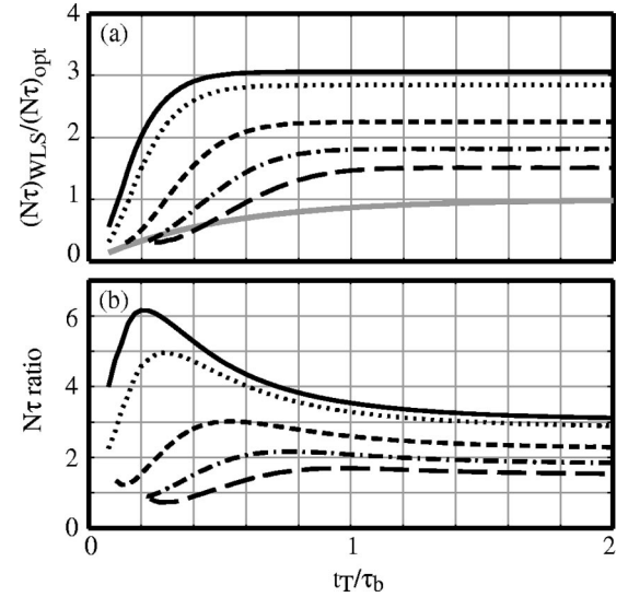
FIG. 5. (a) Values of (N\tau)_{\text{WLS}} for WLS loading as a function of t_T (as a fraction of \tau_b ). The limiting number of atoms that can possibly be loaded into the WLS trap is assumed to be (0.9)N_{\text{lim}} (top curves), or equivalently \tau_1 = \tau_b/10 when the WLS is turned on. The curves represent recovery times 0.035\tau_b (black line), 0.05\tau_b (dotted), 0.1\tau_b (short dashed), 0.15\tau_b (dashed-dotted), and 0.2\tau_b (long dashed). The variation of non-WLS number-lifetime product with time (solid gray line) is shown. The calculations assume that for any particular value of t_T , the WLS is turned off at the optimal t_1 (see Fig. 4). The vertical axis is scaled to (N\tau)_{\text{opt}} . (b) The ratios of the upper curves in (a) to the value of N\tau for unmodulated vapor pressure at any given total MOT trapping time t_T .
