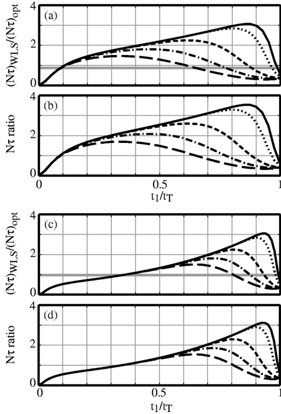
FIG. 4. (a) The calculated products (N\tau)_{\text{WLS}} in units of (N\tau)_{\text{opt}} \equiv N_{\text{lim}}\tau_b/4\alpha , the maximum value that can be achieved with unmodulated vapor pressures, after a total MOT trapping time of t_T = \tau_b . The Rb-limited lifetime is assumed to quickly decrease to \tau_1 = \tau_b/10 when the WLS is turned on. The curves show (N\tau)_{\text{WLS}} at varying times t_1 (as a fraction of t_T ), the point in the MOT loading cycle at which the WLS is turned off, with the remaining time in the cycle ( t_T - t_1 ) permitting recovery of the Rb partial pressure with a time constant of 0.035\tau_b (black line), 0.05\tau_b (dotted), 0.1\tau_b (short dashed), 0.15\tau_b (dashed-dotted), and 0.2\tau_b (long dashed). N\tau for unmodulated vapor pressure is shown as a solid gray line, after a loading time of \tau_T = \tau_b . [Note that for this value to equal (N\tau)_{\text{opt}} , an infinite loading time would be needed.] (b) The ratios of the upper curves in (a) to the value of N\tau for unmodulated vapor pressure after a MOT trapping time of \tau_T = \tau_b . (c,d) Same as for (a) and (b), with a total loading time of t_T = 2\tau_b . Graphs (c) and (d) look nearly identical because N\tau for unmodulated partial pressures is nearly equal to (N\tau)_{\text{opt}} after loading for t_T = 2\tau_b . The four graphs (a)–(d) shown in this figure demonstrate that for a given recovery time and MOT trapping time ( t_T ), there is an optimal WLS duration ( t_1 ) given by the maximum point on the plotted curves.
