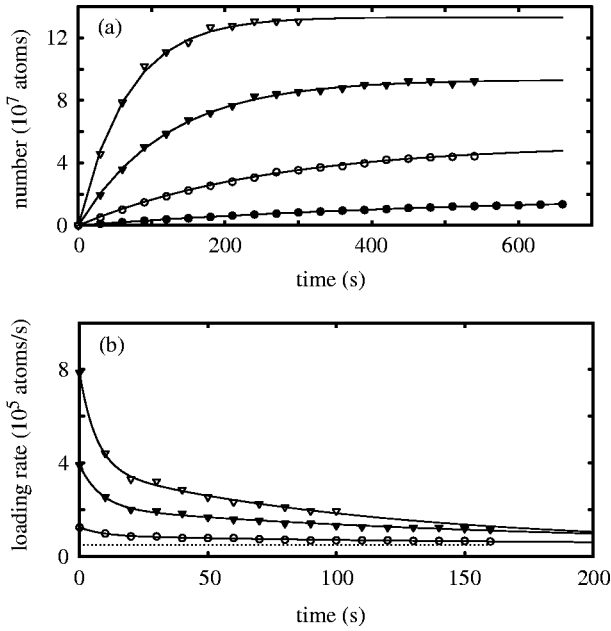
FIG. 2. (a) Comparison of trap loading with and without the additional external white light source. (b) Trend of the loading rate as a function of time after the WLS is turned off. The lower dashed line shows the loading rate before the WLS was turned on. For both (a) and (b), open triangles represent a WLS intensity of \sim 10 W/cm 2 , closed triangles represent a WLS intensity of \sim 5 W/cm 2 , and the open circles represent a WLS intensity of \sim 2 W/cm 2 . The closed circles in (a) represent loading without the WLS. See Table I for a numerical summary of the data shown in these plots.
