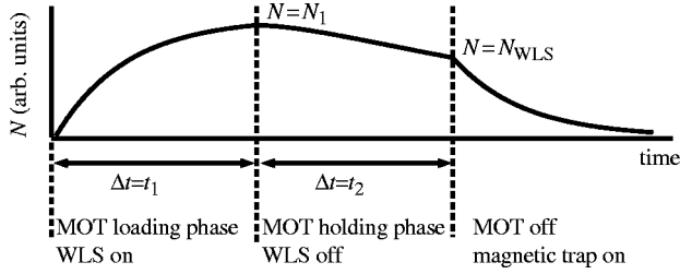
FIG. 3. The timing sequence used in the experiment and in the calculations. The plot is a representation of the number of trapped atoms as a function of time. The dashed lines separate the different stages of trap loading and holding. The number of trapped atoms at the end of the MOT loading and holding phases is given above the N vs time curve. The states of the MOT and the WLS are also listed for the time intervals t_1 and t_2 . After the MOT holding phase, at time t_T = t_1 + t_2 , N_{\text{WLS}} atoms are assumed to be loaded from the MOT into a magnetic trap.
