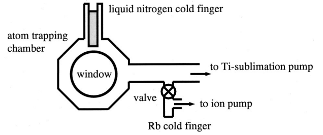
FIG. 1. An illustration of our apparatus. The MOT was formed in the atom trapping chamber, and the WLS light entered into the chamber through a window.
