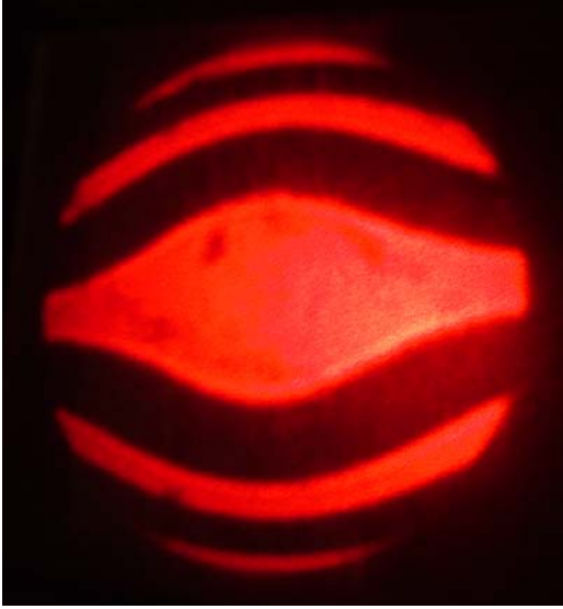
Ronchi Test –Near paraxial focus
