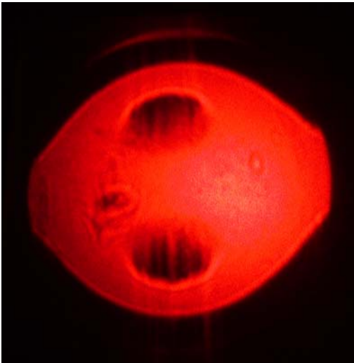
Ronchi Test –Near circle of least confusion
