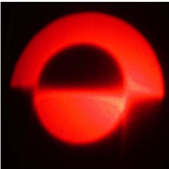
Foucault Test –Near circle of least confusion
