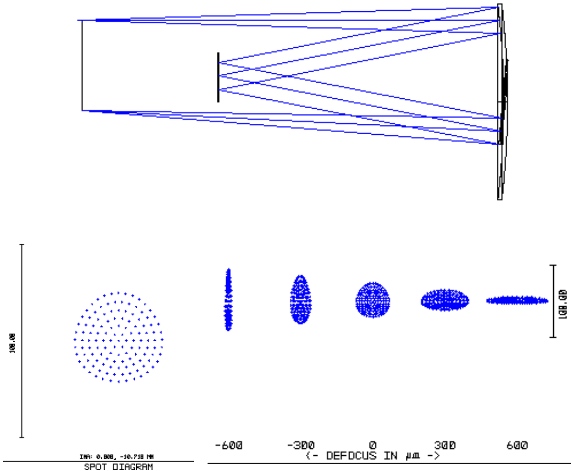
Figure 1. Zemax layout of the spectrometer showing the spot diagram.
