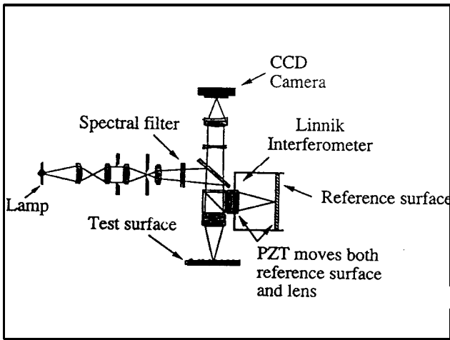
Figure 1. Schematic representation of an optical profiler.
