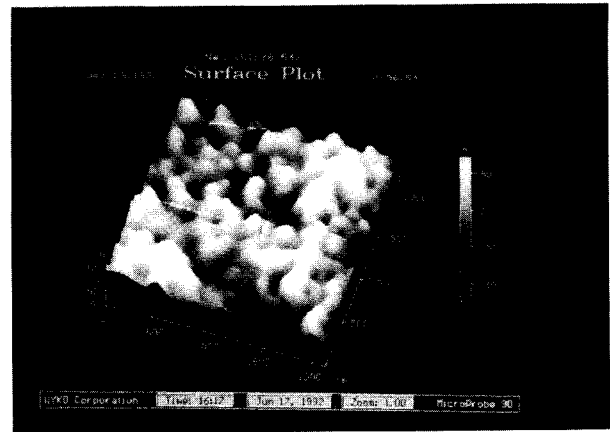
Figure 22. A 2x2 \mu\text{m} image taken on a chemically etched silicon sample with the SPM.
