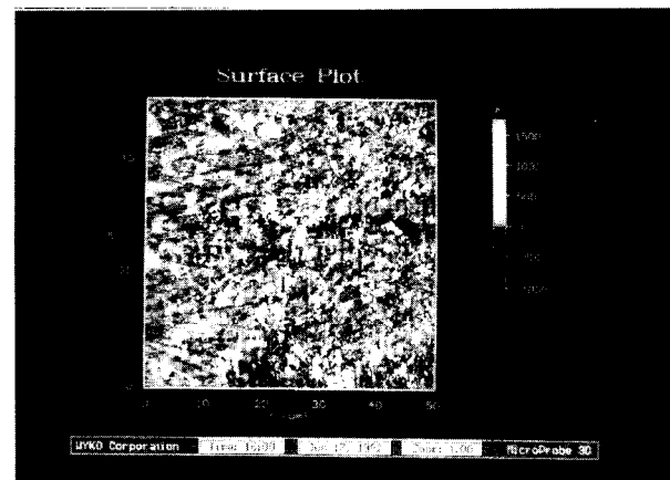
Figure 16. A 50x50 \mu\text{m} image taken on an ABS of a magnetic head sample with the SPM.
