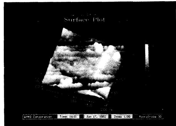
Figure 18. A 2x2 \mu\text{m} image taken on an ABS with the SPM.
