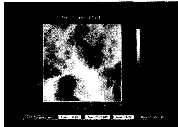
Figure 20. A 50x50 \mu\text{m} image taken on a chemically etched silicon sample with the SPM.
