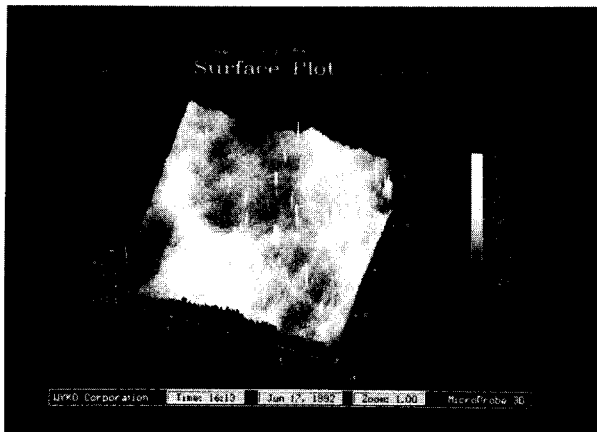
Figure 21. A 20x20 \mu\text{m} image taken on a chemically etched silicon sample with the SPM.
