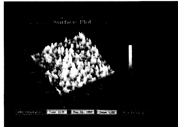
Figure 26. A 2x2 \mu\text{m} image taken on a thin polysilicon film on silicon with the SPM.
