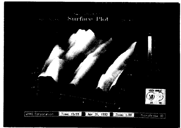
Figure 6. A 6.5x6.5 \mu\text{m} image taken on a magnetic disk with the SPM.
