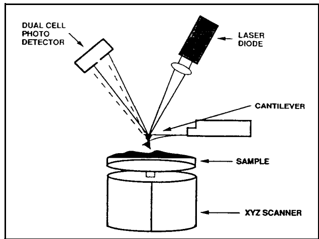
Figure 2. Schematic representation of a scanning force microscope.
