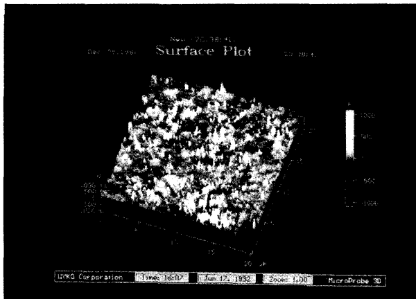
Figure 17. A 20x20 \mu\text{m} image taken on an ABS with the SPM.
