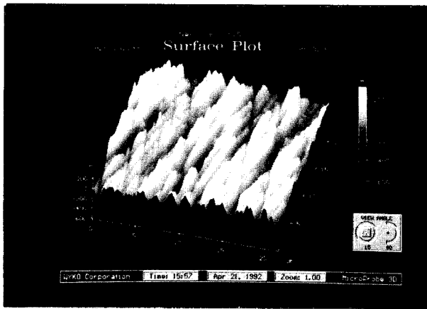
Figure 5. A 21x21 \mu\text{m} image taken on a magnetic disk with the SPM.
