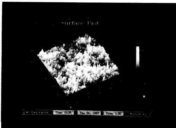
Figure 9. A 20x20 \mu\text{m} image taken on a magnetic tape with the SPM.
