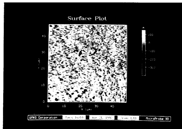
Figure 12. A 50x50 \mu\text{m} image taken on a glass sample with the SPM.
