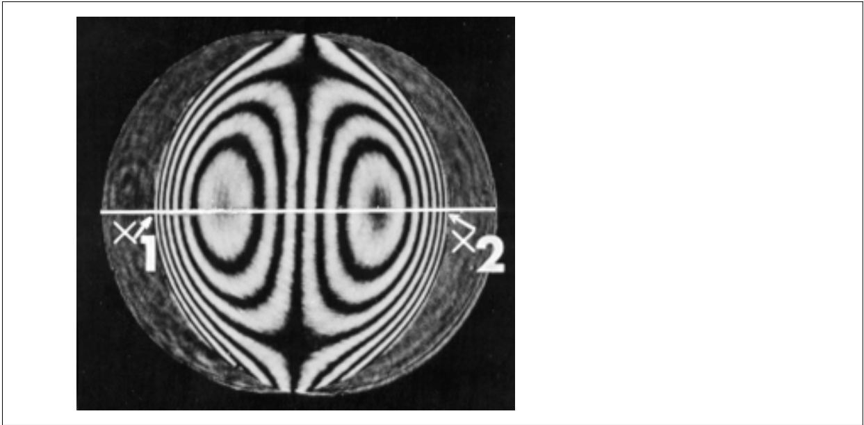
Figure 1. Lateral shear interferogram showing central scan line parallel to the direction of shear.
