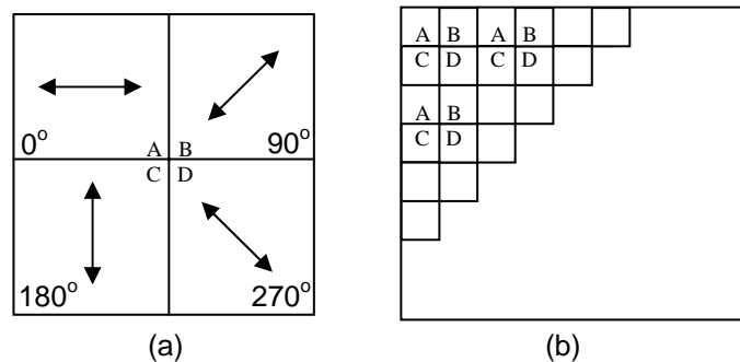
Fig. 2 Phase filter. (a) 4 polarizer elements giving 0, 90, 180, and 270 degree phase shifts. (b) Phase filter made up of array of 4 polarizer elements.
