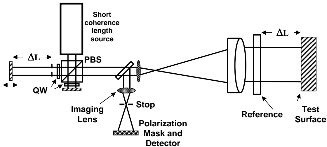
Figure 15. Simultaneous phase-shifting Fizeau – short coherence length source.
