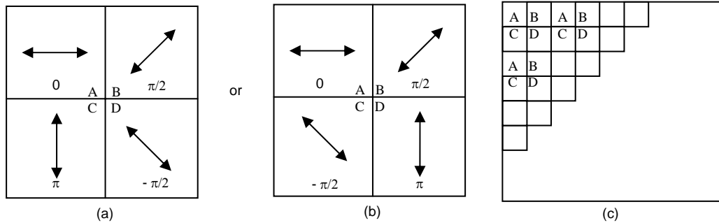
Figure 9. Phase filter. (a) 4 polarizer elements giving 0, 90, 180, and -90 degree phase shifts. (b) 4 polarizer elements giving 0, 90, -90, and 180 degree phase shifts. (c) Phase filter made up of array of 4 polarizer elements.
