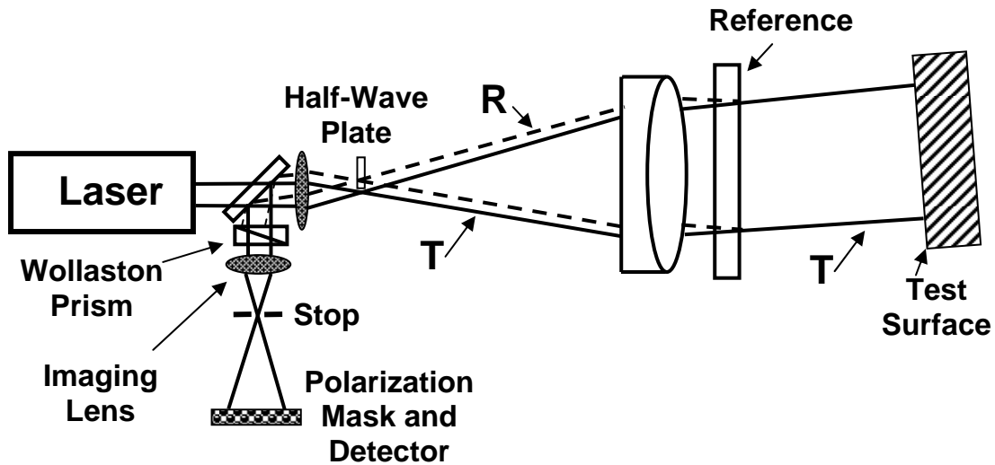
Figure 14. Simultaneous phase-shifting Fizeau – Large tilt between reference and test.
