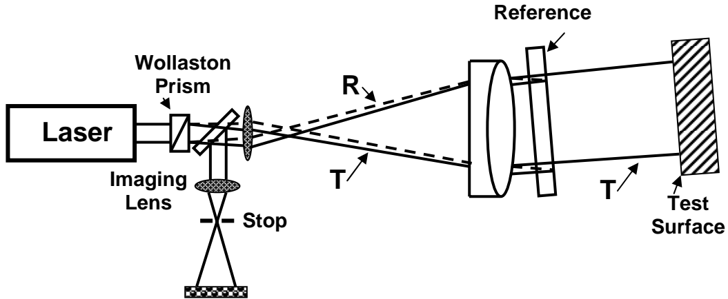
Figure 13. Simultaneous phase-shifting Fizeau – Large tilt between reference and test (Two source beams).
