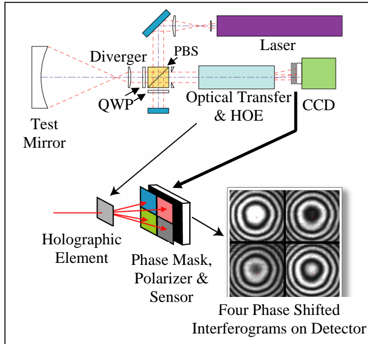
Fig. 2. Simultaneous phase-shifting interferometer (PhaseCam).
