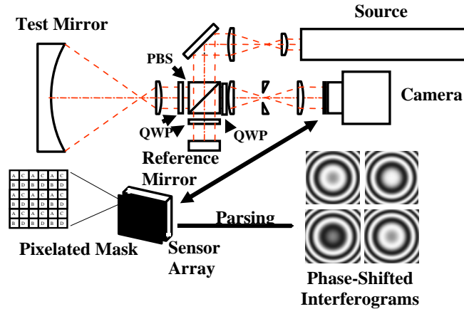
Figure 11. Interferometer Configuration
