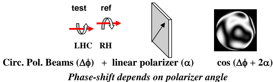
Figure 8. Use of polarizer to introduce phase shift between test and reference beams.
