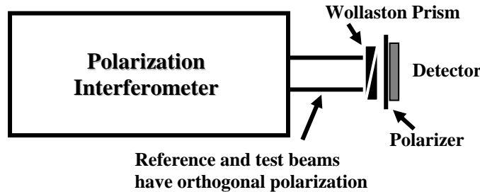
Figure 7. Use of Wollaston prism to produce carrier fringes.
