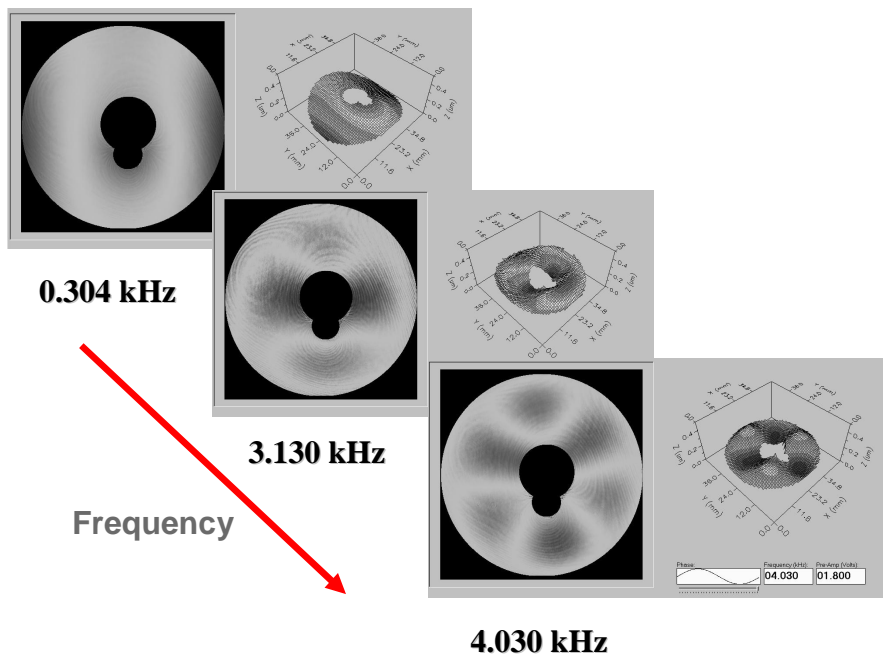
Figure 10. Vibrational modes of a disk.
