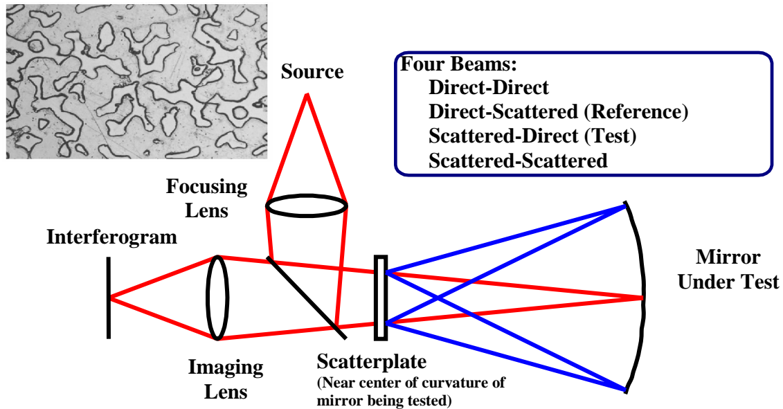
Figure 1. Scatterplate Interferometer for Testing Concave Mirrors.
