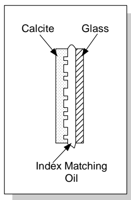
Fig. 5. Birefringent scatterplate.
