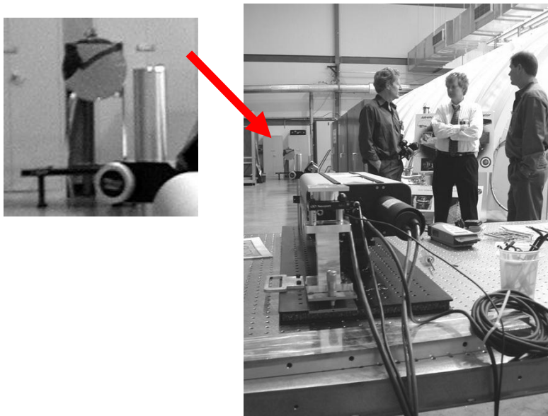
Figure 9. Use of PhaseCam to test a 0.5 meter diameter, 20 meter ROC mirror without any vibration isolation.
