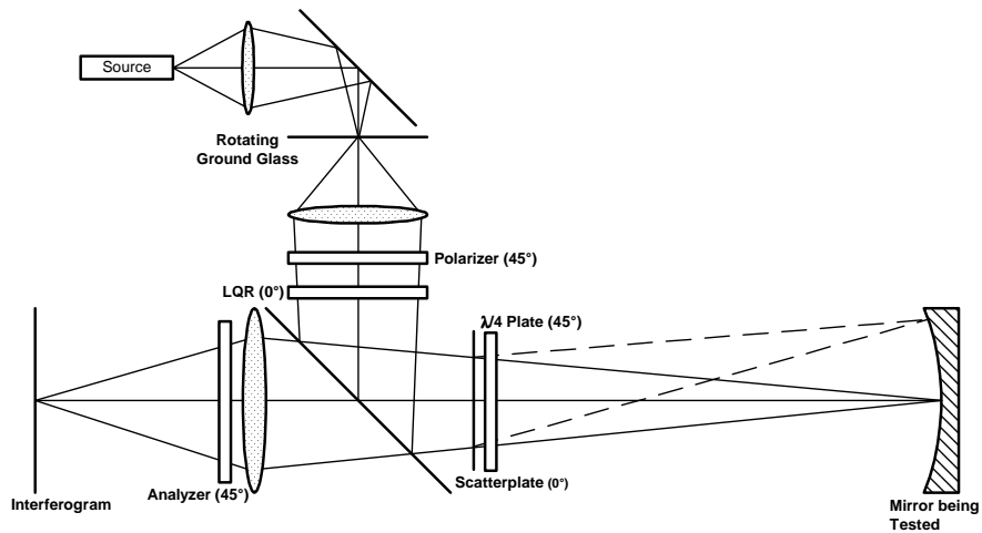
Fig. 6. Phase-shifting scatterplate interferometer.
