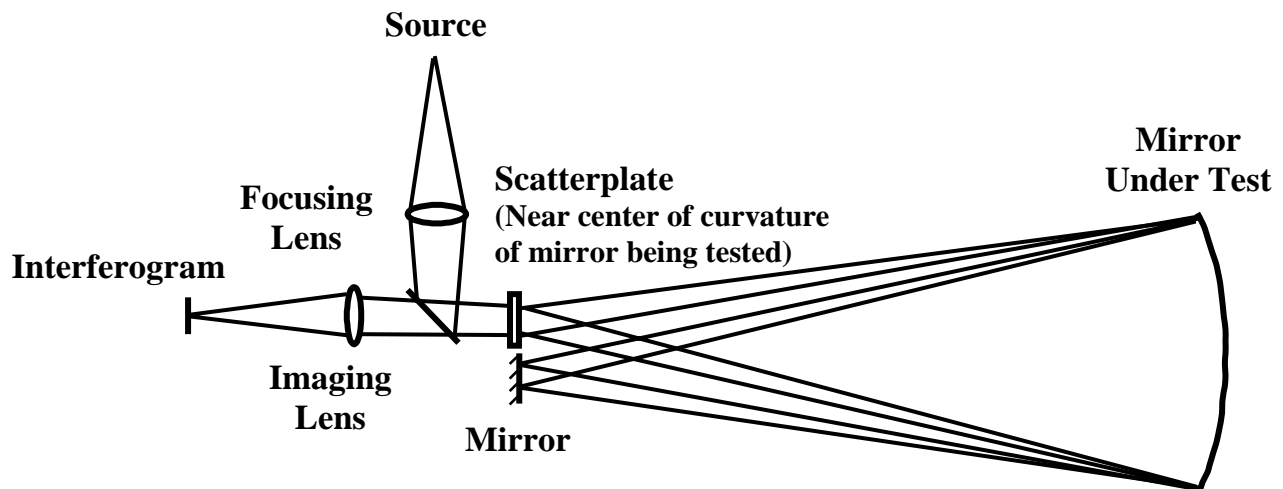
Figure 4. Scatterplate Interferometer insensitive to tip-tilt and piston vibration.
