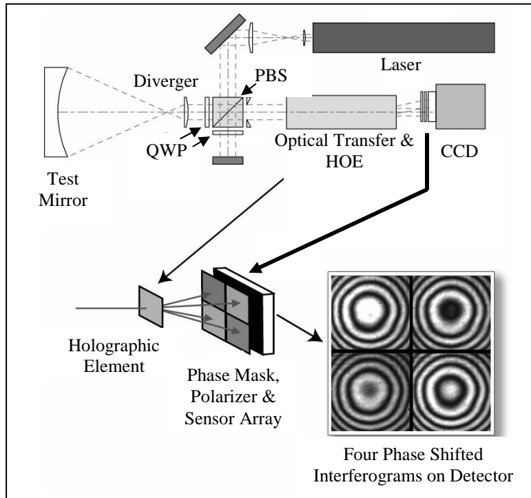
Fig. 8. Single shot interferometer (PhaseCam) showing the beam divider and phase shifting mask.
