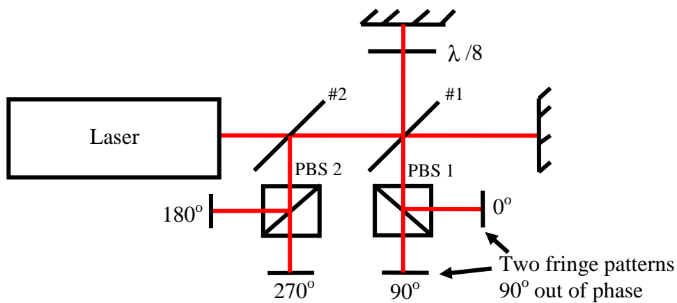
Figure 7. Simultaneous phase-shifting interferometer.
