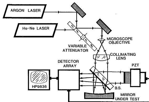
Fig. 4. Experimental setup for the TWLPSI.
