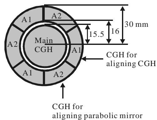
Fig. 6: CGH composition
