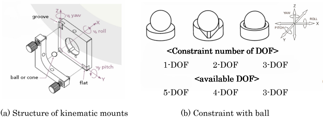
Figure.4.5 Principle of kinematic mount [1]
