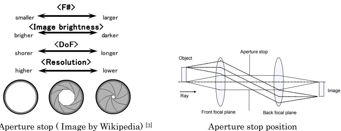
Figure4.3 Aperture stop
