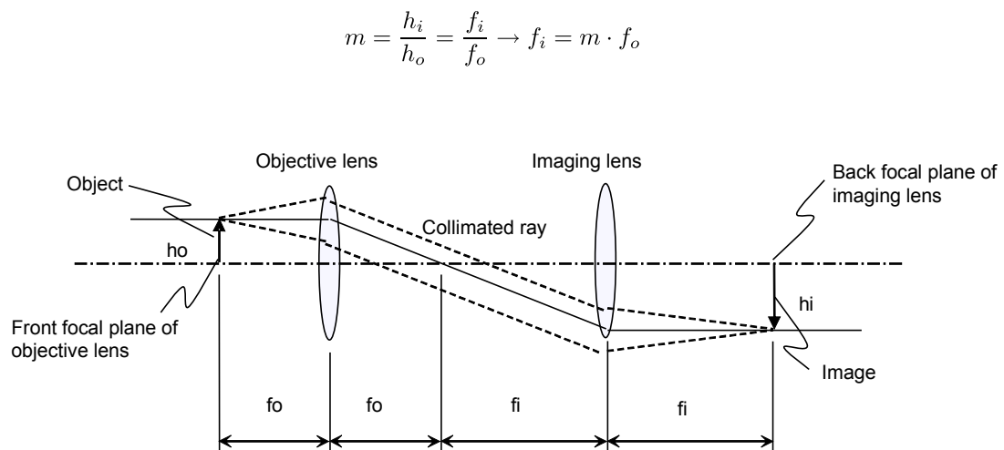
Figure. 3.1 The fundamental optical system with 2 lenses
