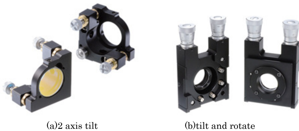
Figure.4.4 Kinematic holder (Image by SIGMA KOKI CO. LTD) [6]
