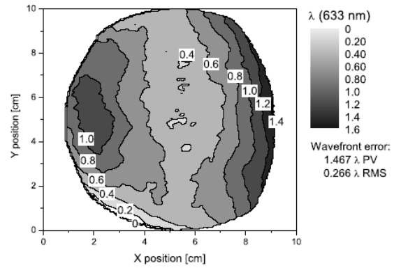
(a) Wavefront at ambient temperature (265 K).
